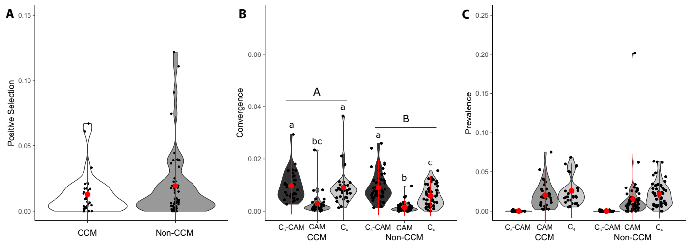
FIGURE 4. Violin plots of (A) the number of sites identified to be under positive selection in carbon concentrating mechanism (CCM) and non-CCM gene families, standardized by sequence length, (B) the total number of independent origins of residues in C 3 -CAM, CAM, and C 4 species that lacked origins in C 3 species in CCM and non-CCM gene families, standardized by sequence length and the number of species represented in each pathway, and (C) the number of prevalent sites (see Fig. 3 legend) for C 3 -CAM, CAM, and C 4 species in CCM and non-CCM gene families, standardized by sequence length. No significant differences between groups are observed in panels A and C. In panel B, there are a significantly greater number of independent origins for C 3 -CAM, CAM, and C 4 species overall in CCM genes than in non-CCM genes (indicated by capital letters), and Tukey groups are assigned with lowercase letters to distinguish significant differences between the interaction of photosynthetic pathway and gene type.
